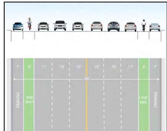
Narrow travel lanes to add bike lanes
